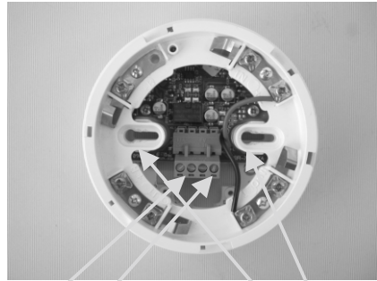
Input / Output Connection Terminals Mounting Screws
